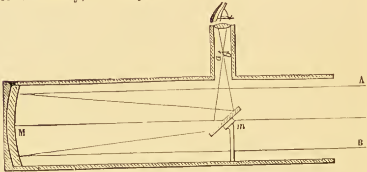
FIG. 82.—Principle of Newtonian reflector.
